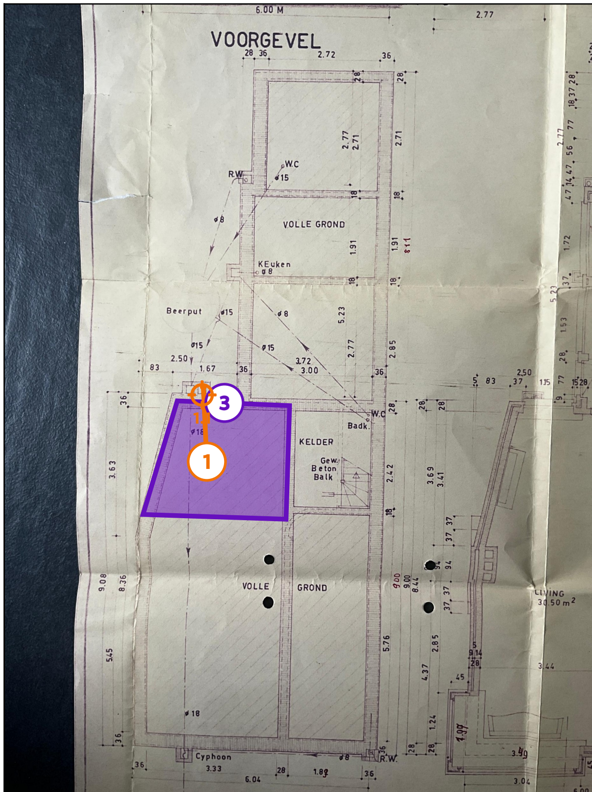
Legende van plan 1.1: plan fundering
